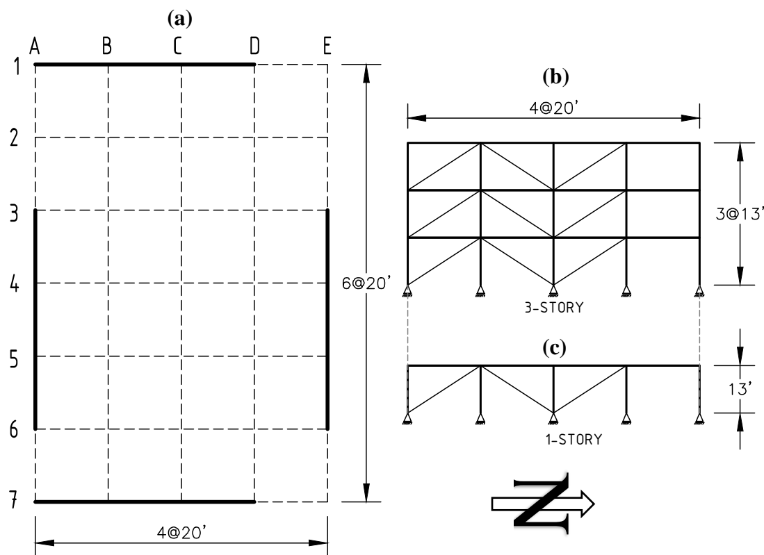
Figure 17. Prototype Buildings. (a) Plan view; (b) 3-Story Elevation view; (c) 1-Story Elevation view
