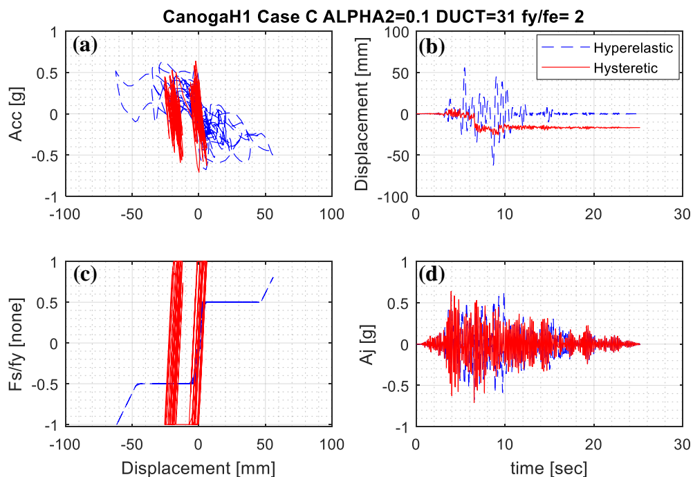
Figure 42. CASE C. (a) Acc. Vs Disp.; (b) Disp. vs. time; (c) normalized brace force vs. Displ.; (d) Acc. vs. time.
