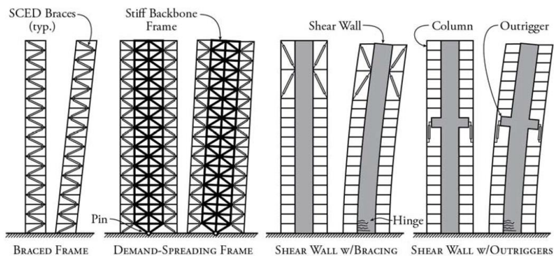
Figure 11. Potential Tall Building Configurations using SCED Braces presented by Erochko and Christopoulos n.d.
