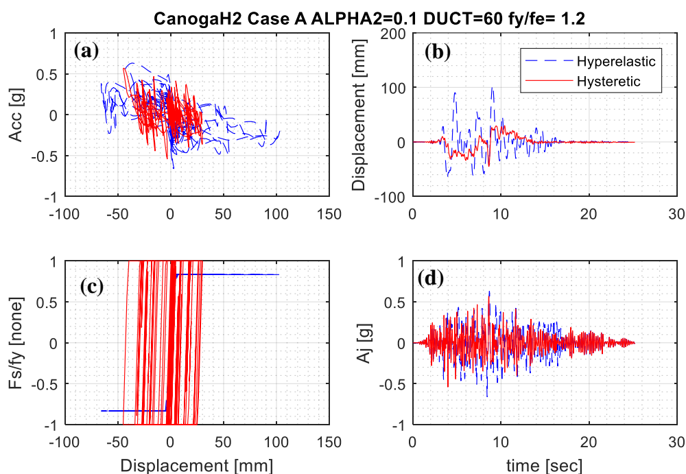
Figure 52. CASE A. (a) Acc. Vs Disp.; (b) Disp. vs. time; (c) normalized brace force vs. Displ.; (d) Acc. vs. time.
