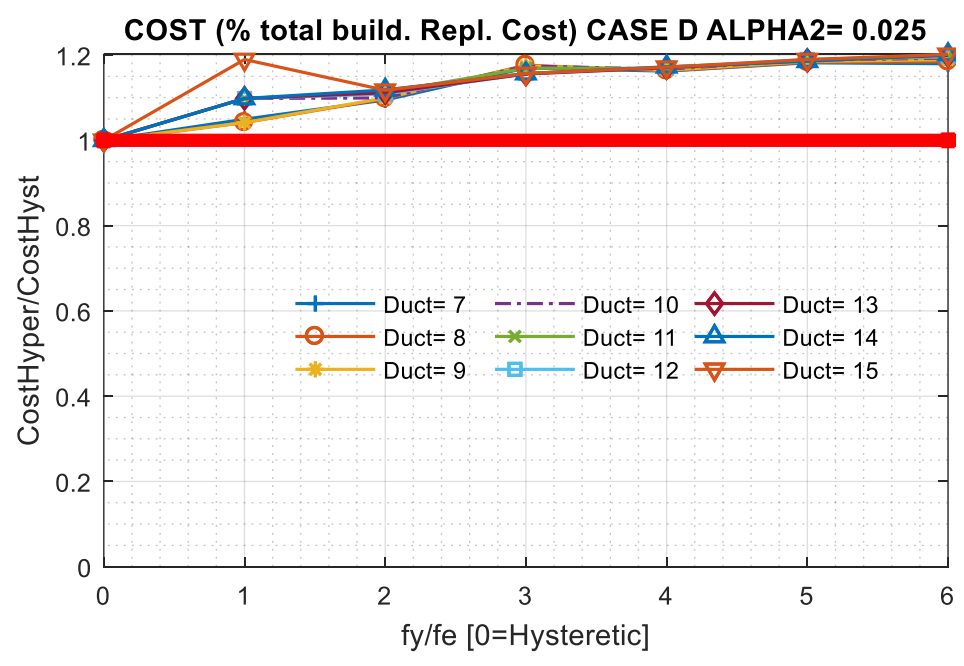
Figure 36. CASE D- \alpha_2=0.025 ; Normalized repair cost, ductility, and f_y/f_e ratio.
