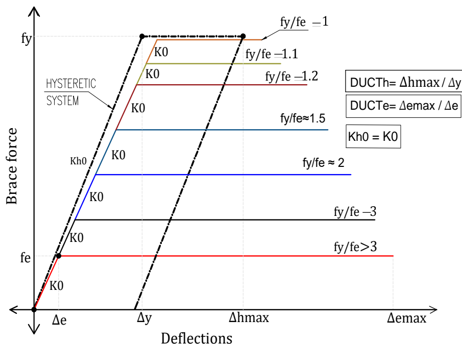
Figure 26. Force-Displacement curve for bilinear hyperelastic systems.
